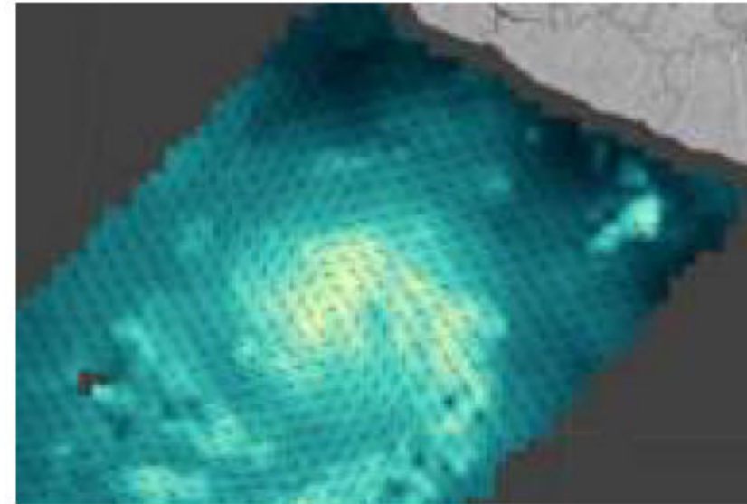
Hurricane Blanca
