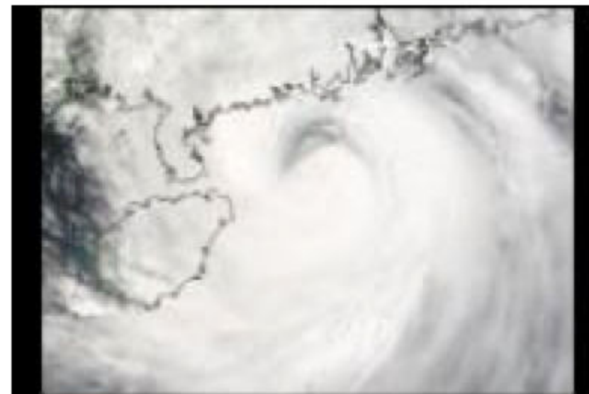
Typhoon Prapiroon
